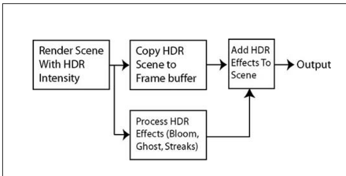
Figure 8.1 Diagram of the general process used to render high dynamic range effects.
