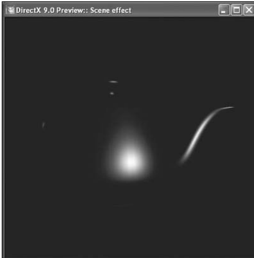
Figure 9.16 Rendering results for your specular lighting shader.
