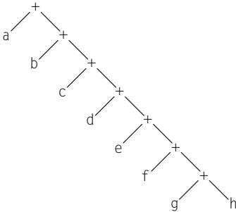
(c) Right-Associative Tree
