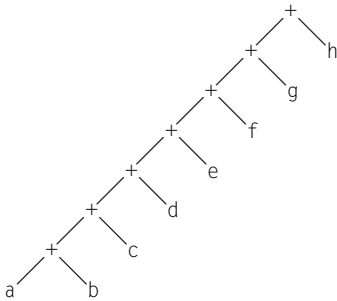
(a) Left-Associative Tree
