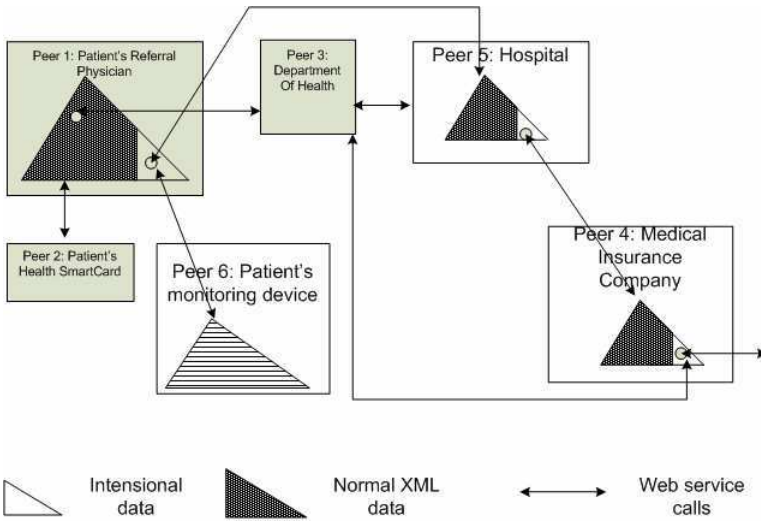
Fig. 4. Models and Relation between peers in EPR
