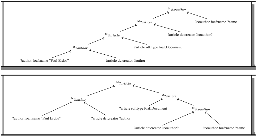
Fig. 10. Left deep and bushy query execution plan
