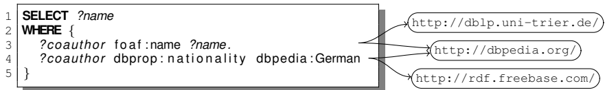
Fig. 8. Query fragment with data source mappings
