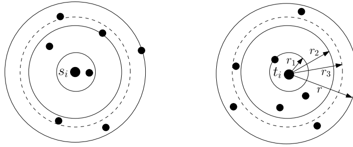
Figure 15.1: An example of the choices of radii r_t around s_i and t_i . The radius r_1 is the smallest such that |B(s_i, r_1)| \geq 2 and |B(t_i, r_1)| \geq 2 . The radius r_2 is the smallest such that |B(s_i, r_2)| \geq 4 and |B(t_i, r_2)| \geq 4 . The radius r is the smallest such that |B(s_i, r)| \geq 8 and |B(t_i, r)| \geq 8 . Since r \geq \frac{1}{4}d_{s_i t_i} , but r_2 is less than this, \hat{t} = 3 , and r_{\hat{t}} = r_3 = \frac{1}{4}d_{s_i t_i} .
