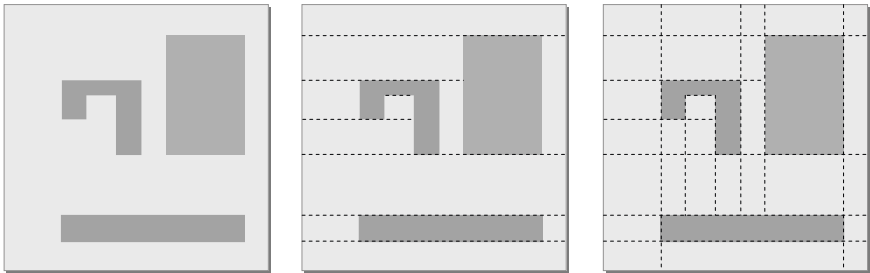
Fig. 5.17 Given a layout area with macro blocks (left), the horizontal (center) and vertical (right) macro-cell edges are extended to form the routing regions.
