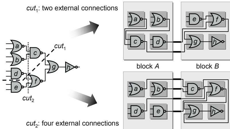
Fig. 2.1 Two different partitions induced by cuts cut_1 and cut_2 , producing two and four external connections, respectively.
