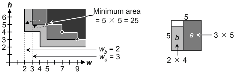
Fig. 3.11 Finding the shapes of the individual blocks from the same top-level floorplan example (Fig. 3.9 and Fig. 3.10) with library blocks a ( 5 \times 3 ) and b ( 2 \times 4 ). The minimum-area floorplan F has w_F = 5 and h_F = 5 (left). The dimensions and locations of the individual blocks a and b (right) are derived by tracing back to the blocks' respective shape functions.
