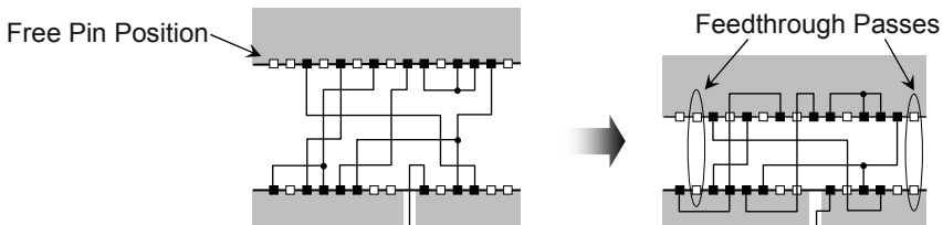
Fig. 6.16 WISER uses free pin positions to reduce the number of channel tracks from four to two [6.10]. Feedthroughs are free vertical routing tracks from top to bottom of a cell that enable connections between adjacent channels. When unused pin locations are located opposite each other on the top and bottom of a channel, feedthroughs result whereby vertical Metal2 is again free to make a connection between adjacent channels. An unused pin location means that there is no Metal1 feature (pin) at that location inside the standard cell, and hence no need for Metal2 to connect to any standard-cell pin. Hence, the Metal2 resource is available.
