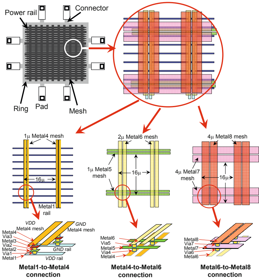
Fig. 3.23 Construction of a mesh power-ground distribution network.
