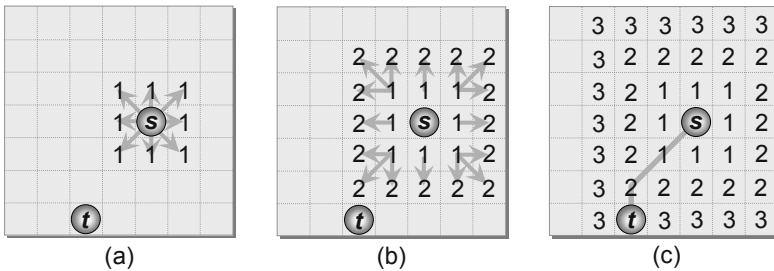
Fig. 7.7 Octilinear maze search with Lee’s algorithm. (a) The initial outward pass from the source node s . (b) The second pass, branching out in all eight directions. (c) The third pass, where the target node t has been found, and a path is traced back from t to s .
