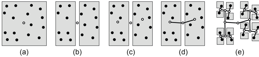
Fig. 7.11 Illustration of the main steps of the method of means and medians (MMM). (a) Find the center of mass (white ‘o’) of the point set S (black ‘o’). (b) Partition S by the median. (c) Find the center of mass for the left and right subsets of S . (d) Route (connect) the center of mass of S with the centers of mass of the left and right subsets of S . (e) Final result after recursively performing MMM on each subset.
