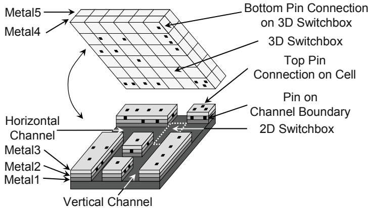
Fig. 5.5 2D and 3D switchboxes in a five-layer process. The cells are internally routed using layers up to Metal3. 2D switchboxes typically exist on layers Metal1, Metal2 and Metal3. Layers Metal4 and Metal5 are connected by a 3D switchbox.
