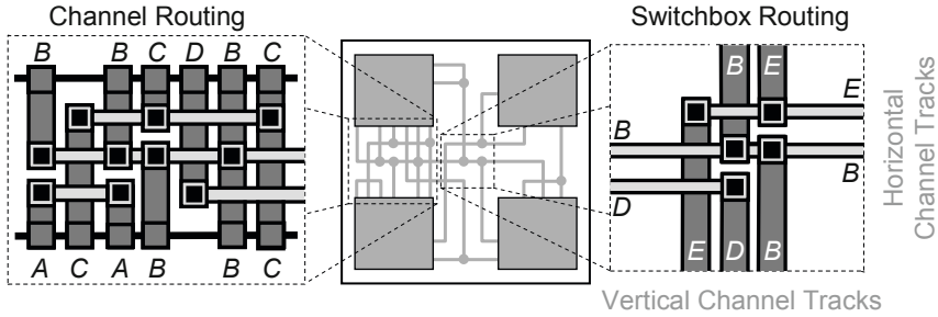
Fig. 6.1 Example of two-layer channel and switchbox routing. The pins of each net A-D are all positioned perpendicular to the channel. Each layer has a preferred direction – one layer has only horizontal tracks and one layer has only vertical tracks. Vias are used if routing a net requires both horizontal and vertical tracks.
