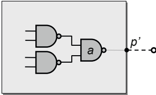
Fig. 4.8 Placement of cell a is close to the terminal p' , which represents a connection to a neighboring partition.
