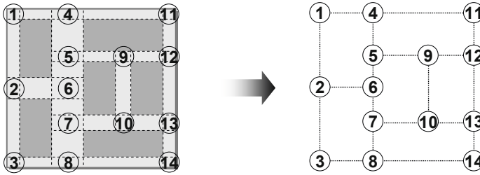
Fig. 5.13 Sample layout with its corresponding switchbox connectivity graph.
