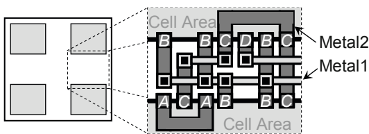
Fig. 6.13 OTC routing with two metal layers. For another example, see Fig. 1.7.
