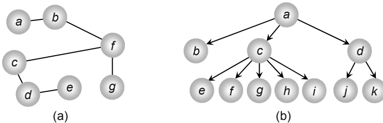
Fig. 1.15 (a) A undirected graph with leaves a, e and g , and maximum node degree 3. (b) A directed tree with root a and leaves b and e-k .
