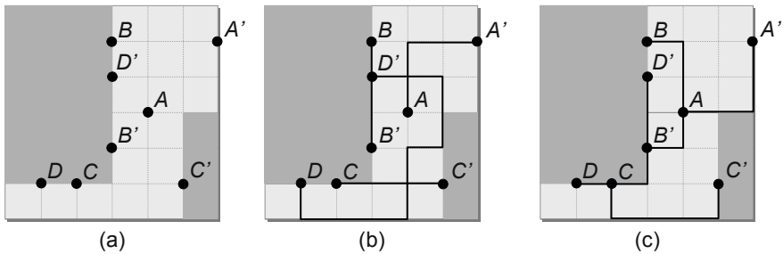
Fig. 5.20 Routing without violations versus rip-up and reroute. Let the net ordering be A - B - C - D . (a) The routing instance with nets A - D . (b) If all nets are routed without allowing violations, net D is forced to detour heavily; the resulting total wirelength is 21. (c) If routes are routed with allowing violations, all nets with violation can be ripped up and rerouted, resulting in lower wirelength. In this example, net A is rerouted with a shortest-path configuration, nets B and C are slightly detoured, and net D remains the same with its shortest-path configuration. The resulting wirelength is 19.
