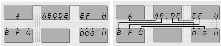
Fig. 5.10 A gate-array design with channel height = 4 (left). If all nets are routed with their shortest paths, the full netlist is unroutable. In one possible routing, net C is remains unrouted (right).
