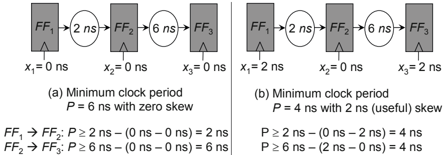
Fig. 7.9 Example of useful skew for clock cycle time reduction. (a) Zero skew results in a 6 ns clock period. (b) Useful skews of 2 ns, 0 ns and 2 ns at x_1 , x_2 and x_3 result in a 4 ns clock period.
