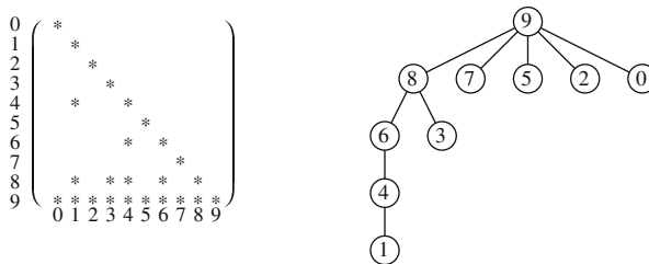
Fig. 7.25 Sparse matrix and the corresponding elimination tree
