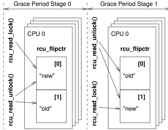
Figure D.61: Preemptible RCU Counter Flip Operation
