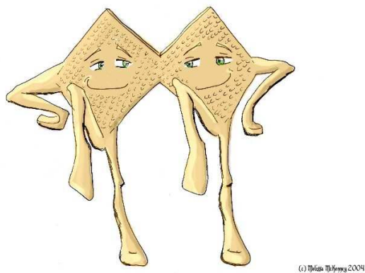
Figure 15.2: Multithreaded Mania
